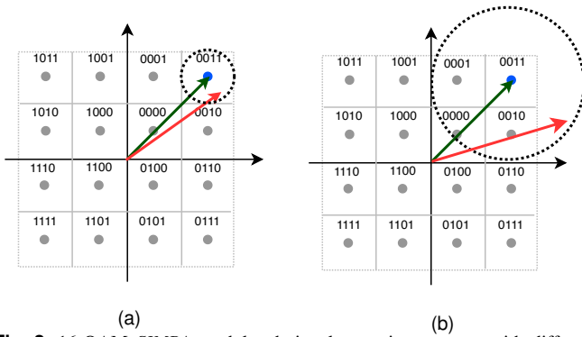
Fig. 2: 16-QAM SIMBA modulated signal reception at users with different channel quality. The transmitted symbol is represented in green, received in red, and noise in black. (a) A high SNR decodes all 4 bits (b) A low SNR user decodes only 2 bits (infer only the quadrant of transmitted sample).
