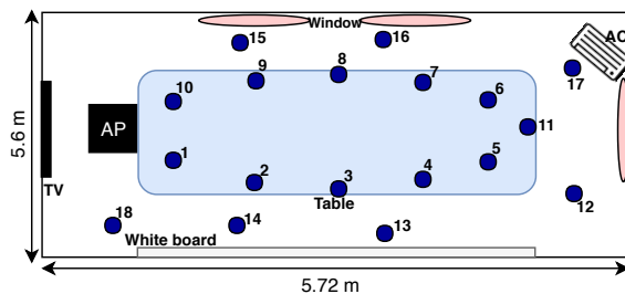
Fig. 6: Experimental floor plan used for measurement of data using WARP-60 testbed.
