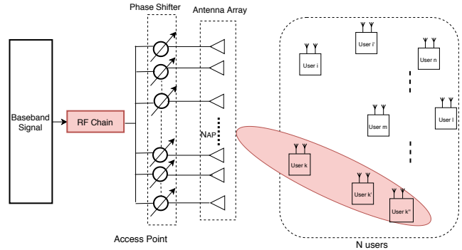
Fig. 1: AP with single RF chain system supporting multiple users
