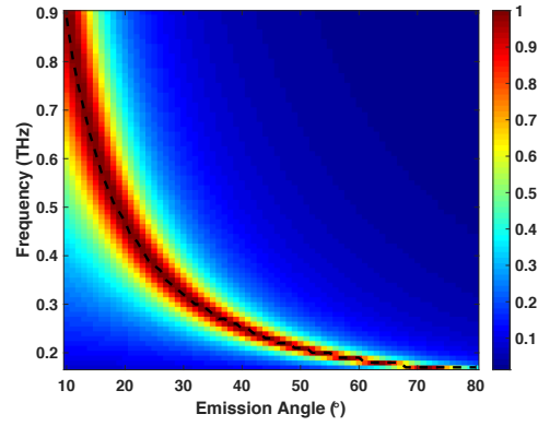
Figure 2: Spectrum-Angle radiation heatmap.
